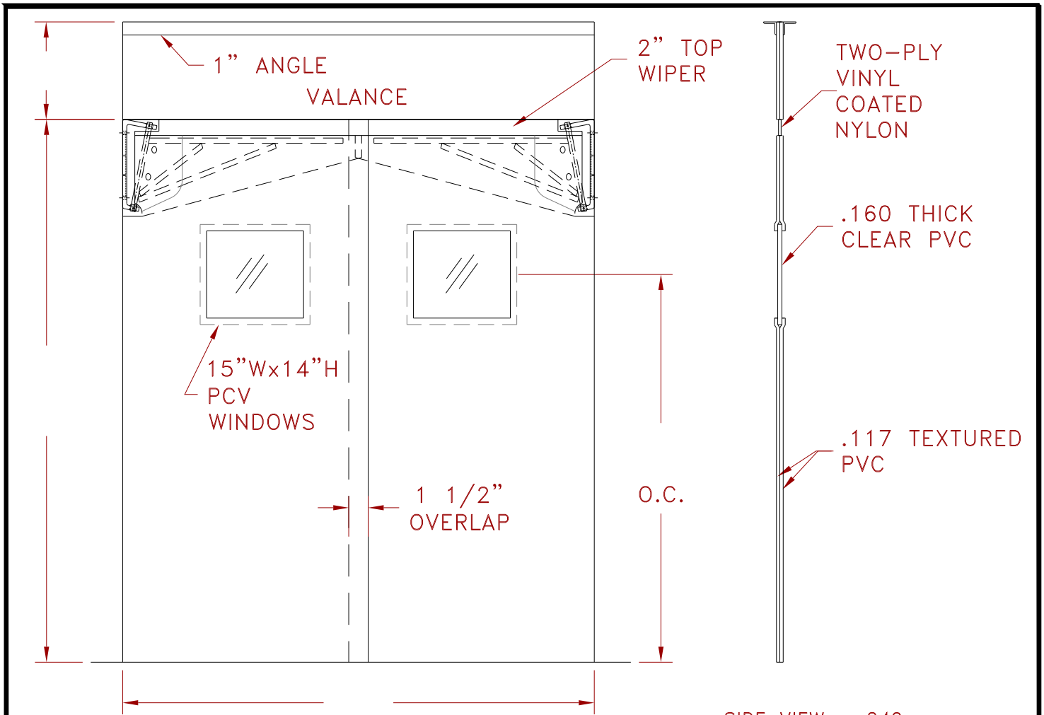
SIDE VIEW - 240
