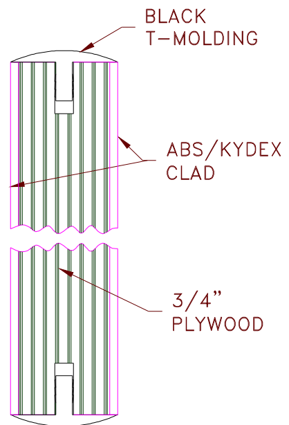
VIEW "AA" (ABS/KYDEX CLAD)
