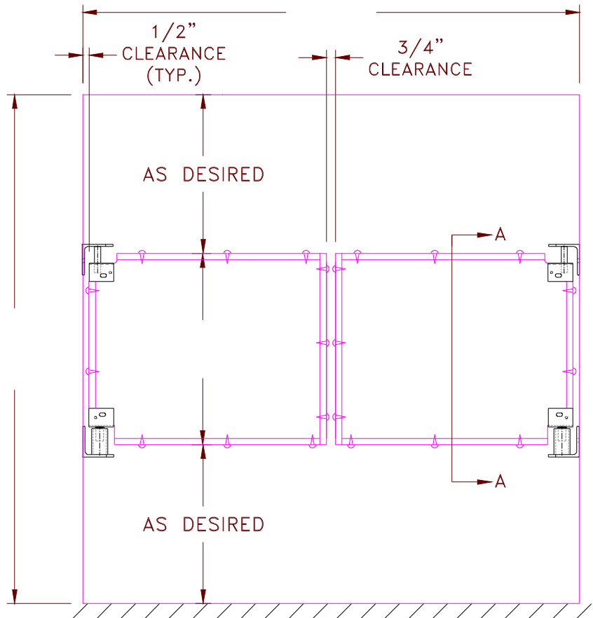
VIEW "AA" (ALUMINUM CLAD)
