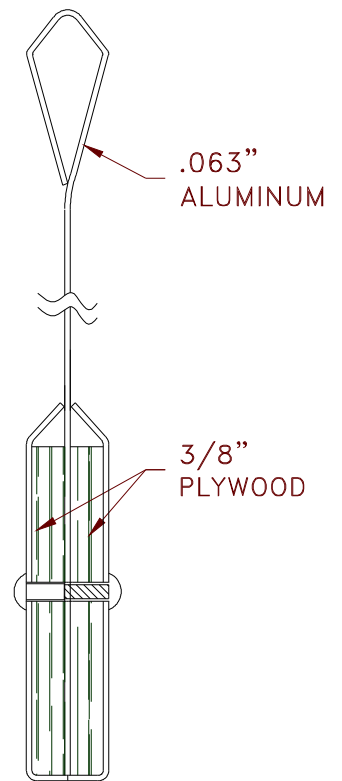
SECTION "AA" OF DOOR
