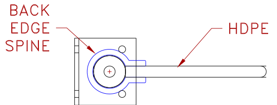
SECTION "AA" OF DOOR
