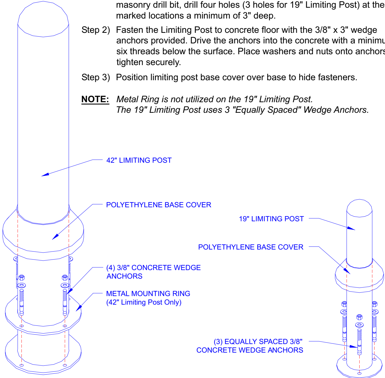
42" Limiting Post
